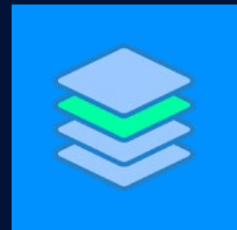
Consensus Layer
